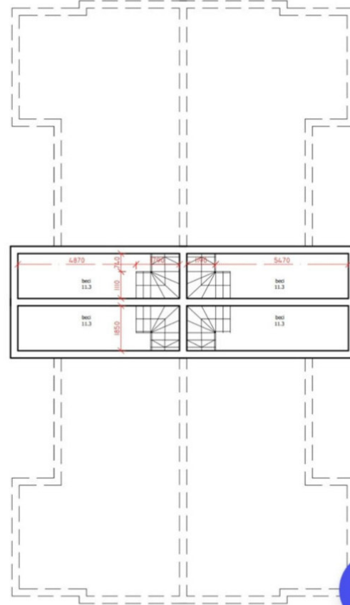
PLAN SUBSOL SC. I-100 SUBSOL APARTAMENT - 11.3M2
