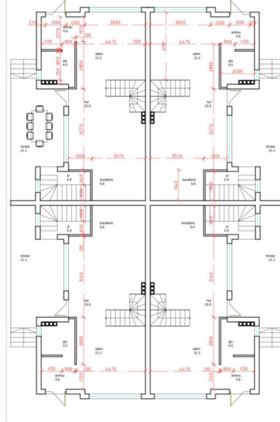
PLAN PARTER SC. 1-100 SPARTER APARTAMENT - 67.8M2
